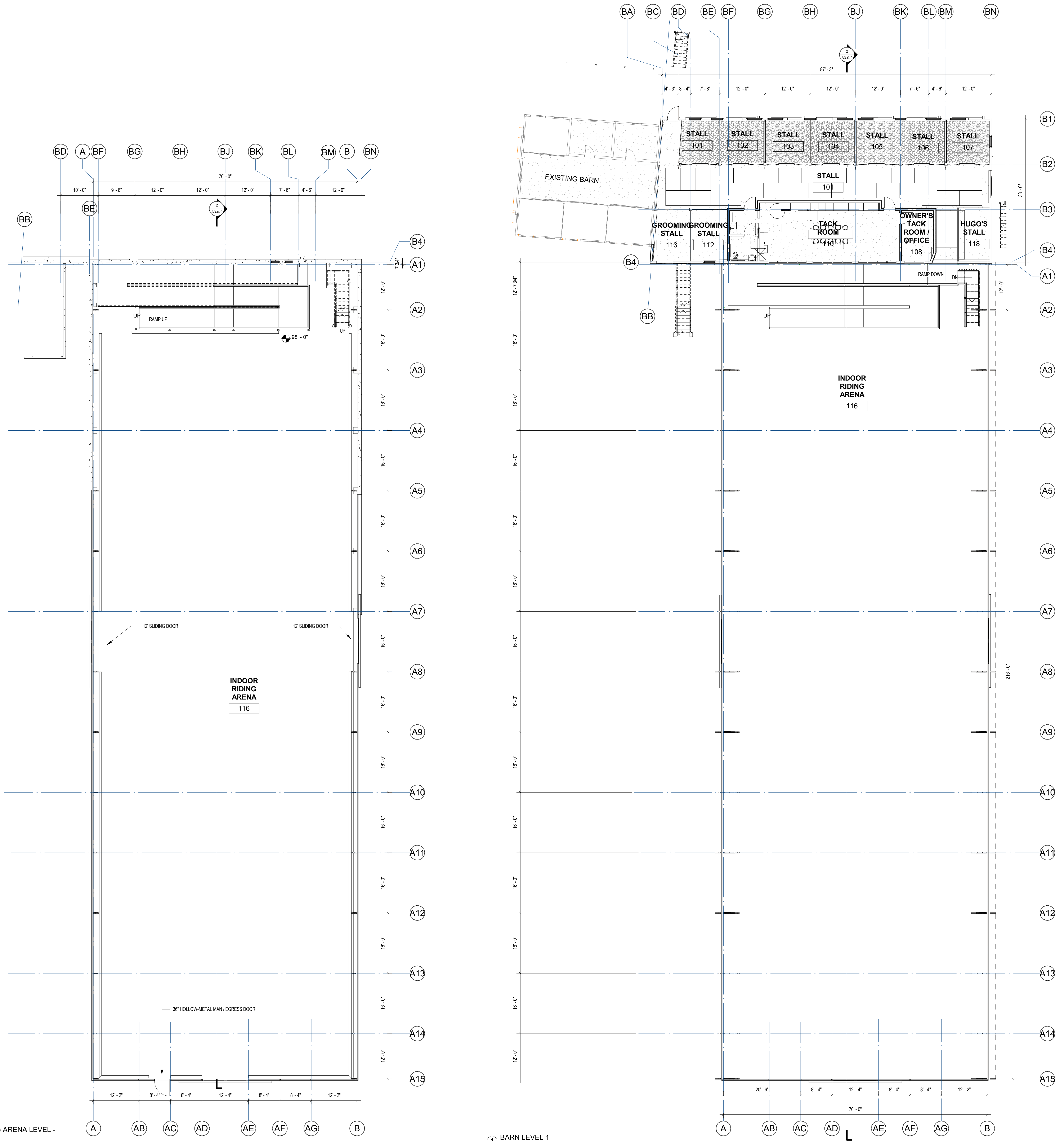
1 BARN LEVEL 1 3/32" = 1'-0"
